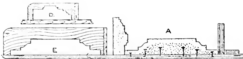
NO. 146.—REVERSE MOULDS FOR PANEL MOULDINGS.
